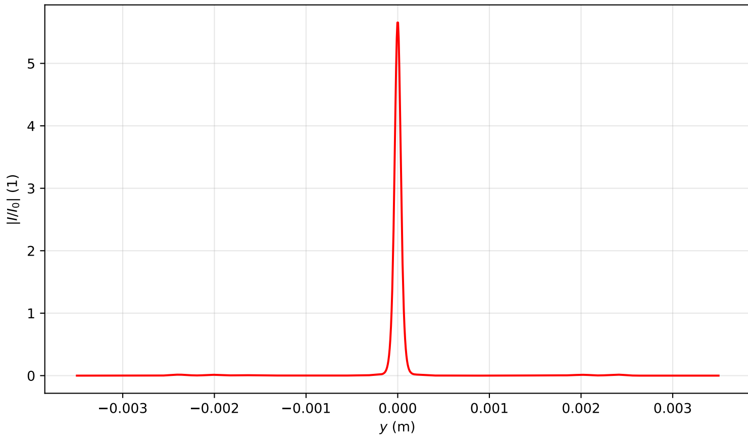
Intensity profile I(x=0, y, z=2.548)/I_0 , P_{in}=9.0P_{cr} , artificial time
